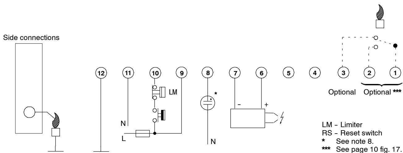
Fig. 13. Connection diagram S4565QD with external ignition circuit
