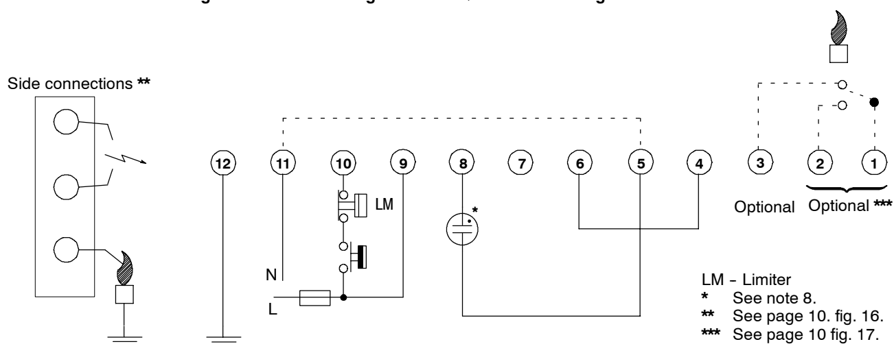
Fig. 14. Connection diagram S4565PD and QD
