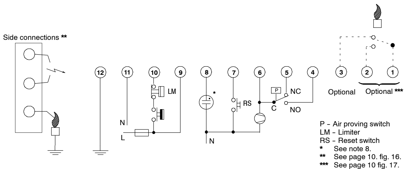
Fig. 12. Connection diagram S4565CD and DD
