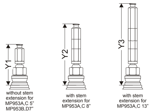
Fig. 5. Stem extensions
