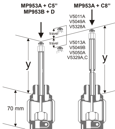
Fig. 7. Extension yoke
