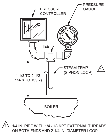
Fig. 2. Steam trap mounting.
