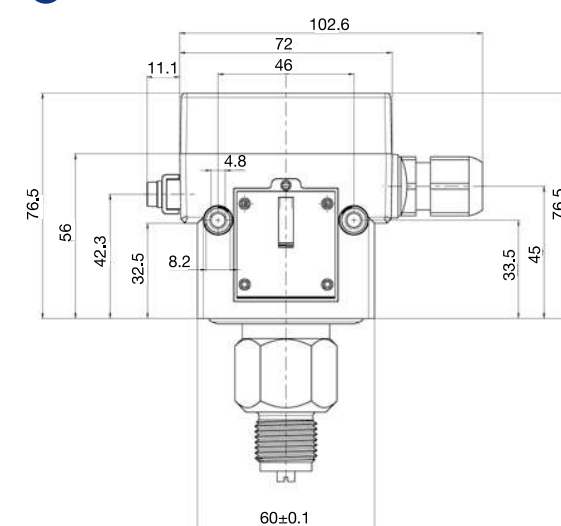
4 Housing 700 (terminal connection Ex-d)
