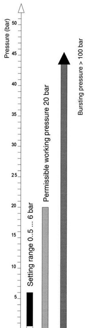
Pressure data for a pressure switch based on the example of DWR625:
