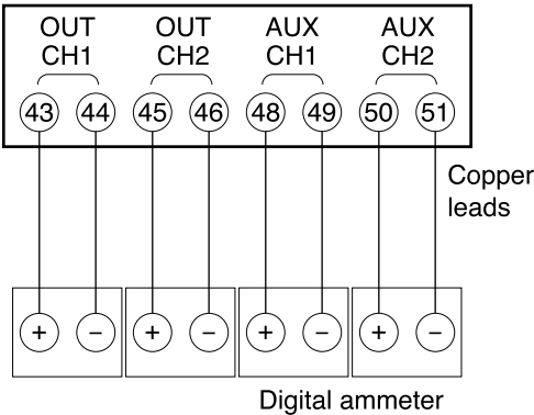
Figure 12-11. Current Outputs
