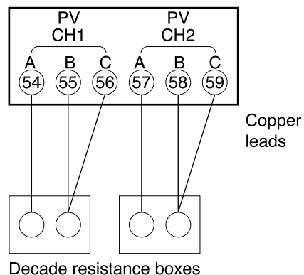
Figure 12-6. RTD Inputs
