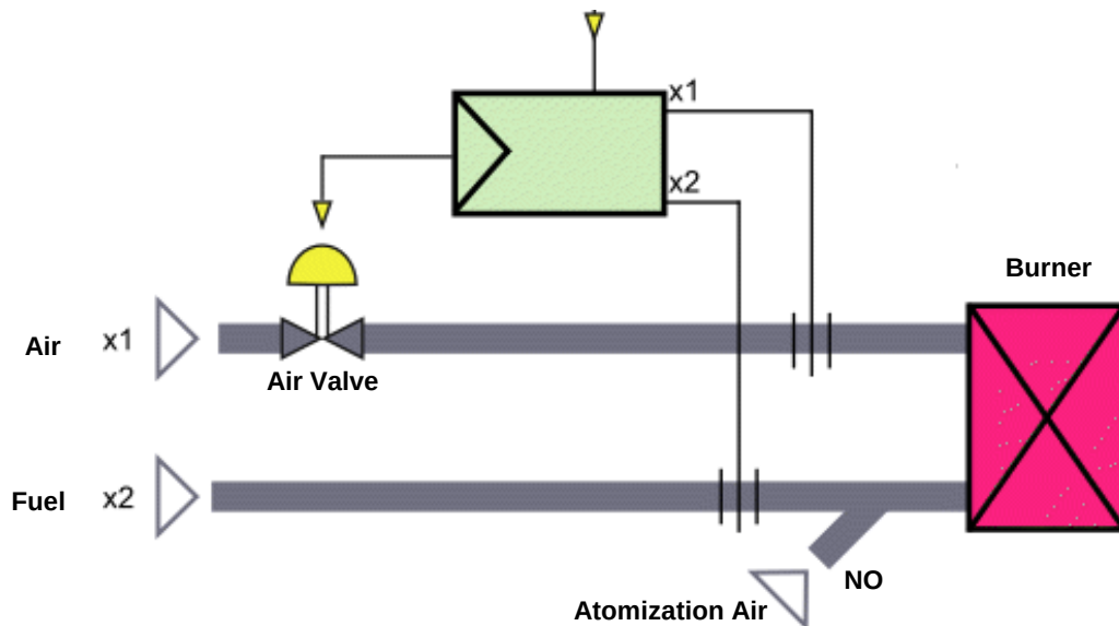
Figure 48. Ratio Control Example
