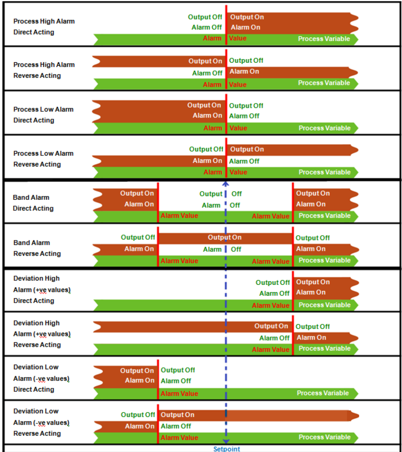
Figure 64. Alarm Operation
