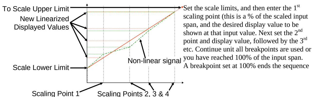
Figure 46. Multi-point Scaling
