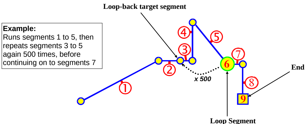
Figure 50. Loop-back Segments
