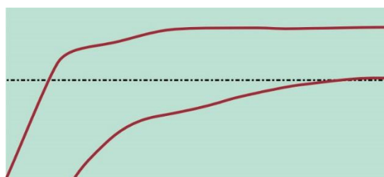
Too Short: Slow to setpoint or offset above/below setpoint
