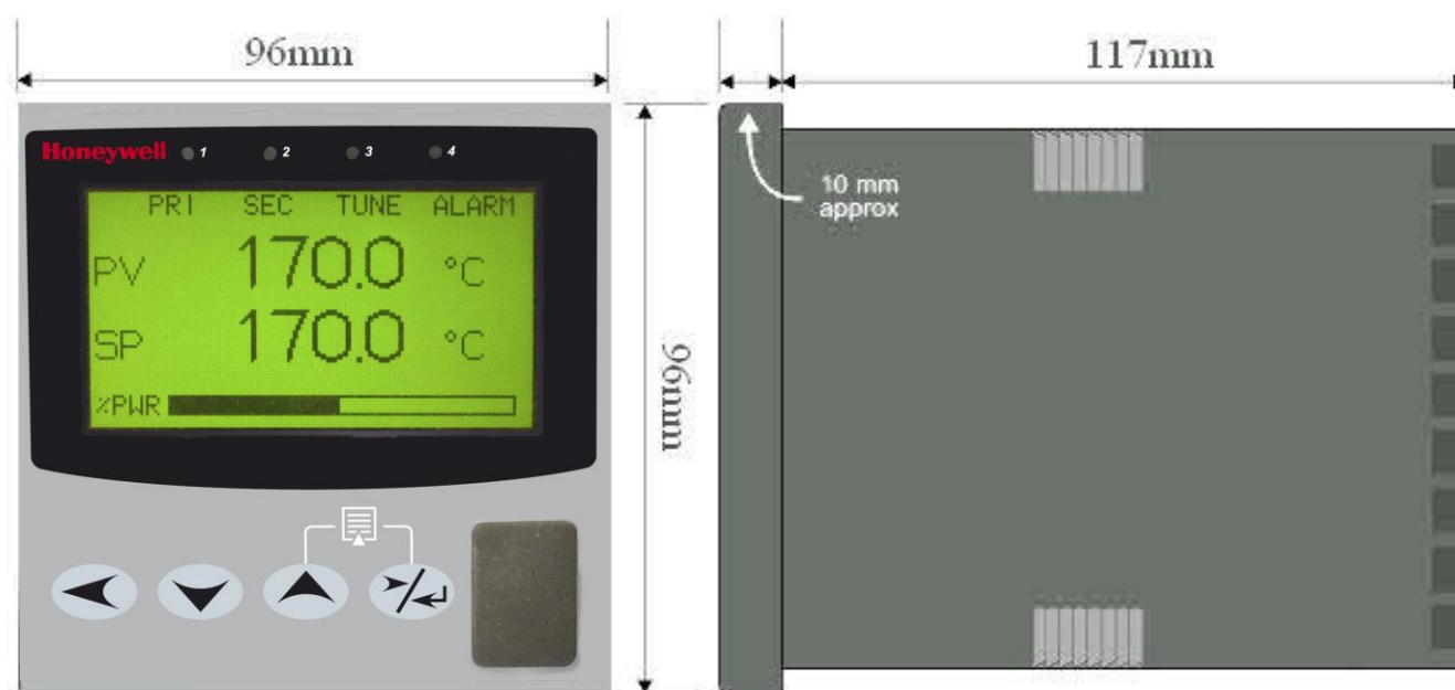
Figure 1. Main dimensions
