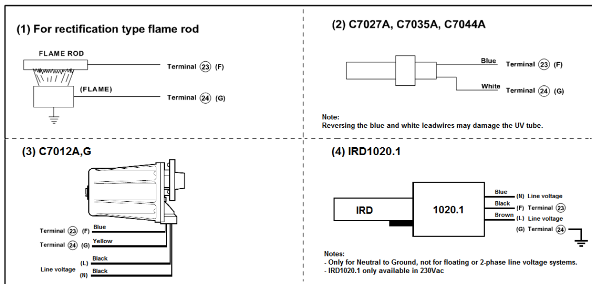
Fig. 4-1: Wiring a flame detector
