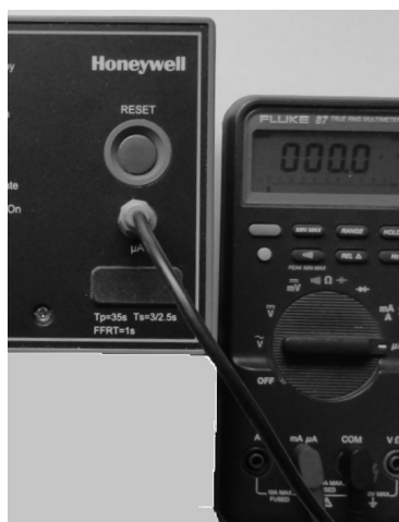
Fig. 4-3: Measuring flame signal with multi meter ( \mu A range selection) using a jack plug.
