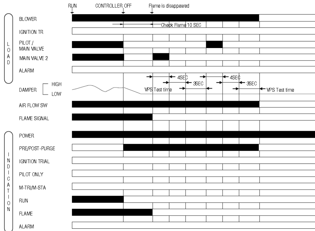
Fig 18b. VPS- post normal operation for DBI configuration.
