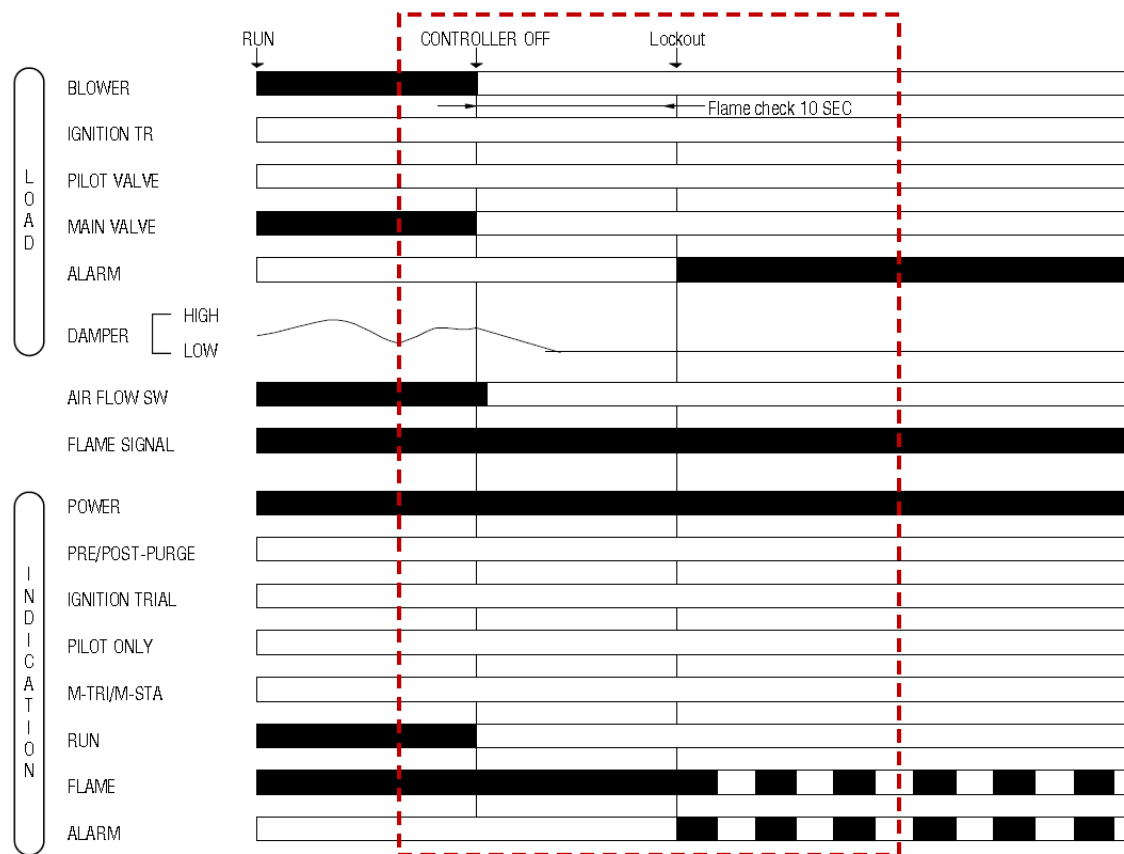
Fig 12b. Flame signal remains present after the end of heat demand: NO-POST-PURGE configuration.
