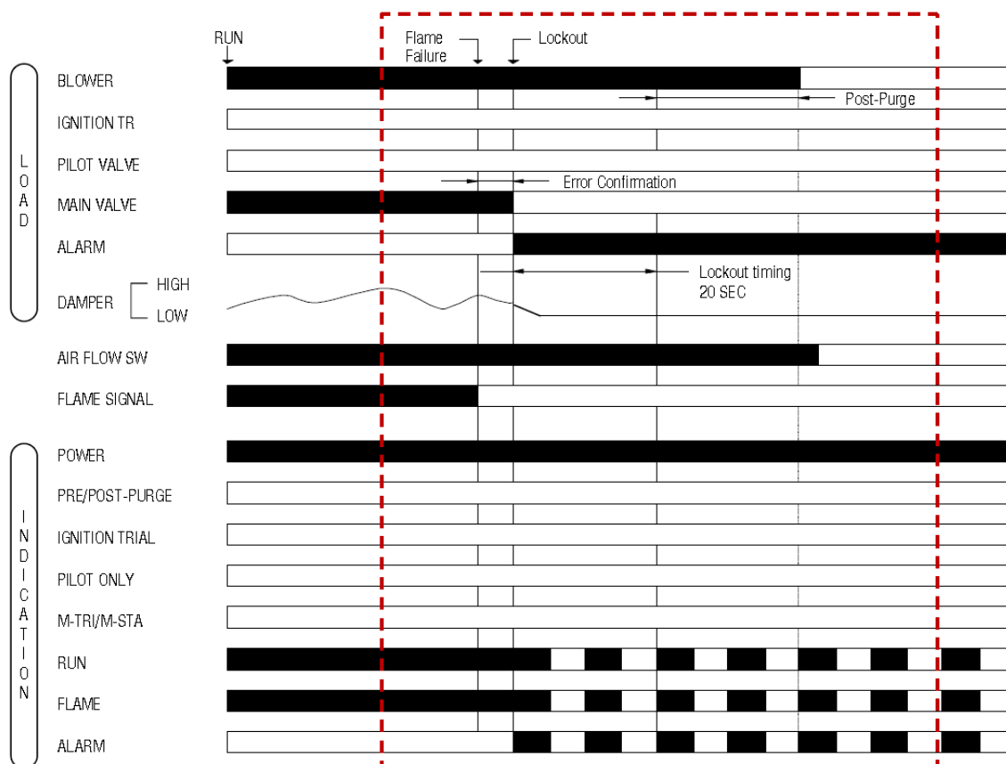
Fig 7a. Flame failure during run period: POST-PURGE configuration.
