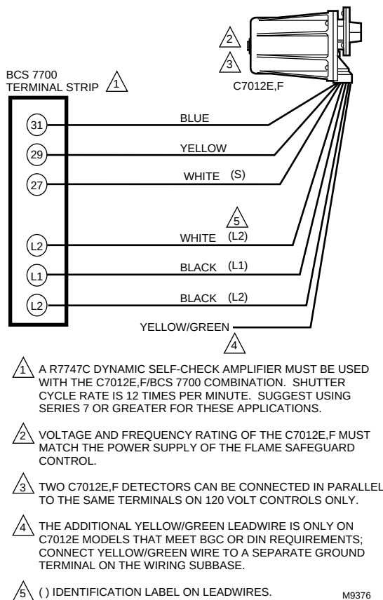
Fig. 14. Wiring diagram for C7012E,F Detectors with BCS 7700 Flame Safeguard controls.
