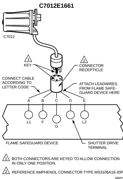
Fig. 16. Wiring connection for C7012E1161 or C7012E1278.
