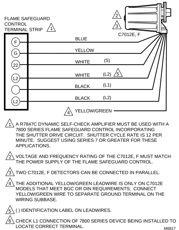
Fig. 15. Wiring diagram for C7012E,F Detectors with 7800 SERIES Flame Safeguard Controls with shutter drive circuitry.
