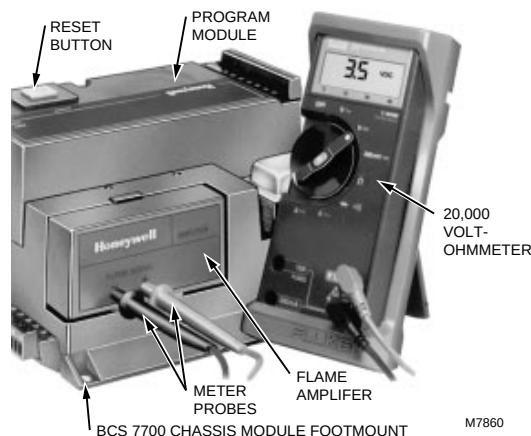
Fig. 18. Measuring voltage flame signal with BCS 7700 controls.
