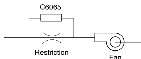
Fig. 2. Air path circuit
