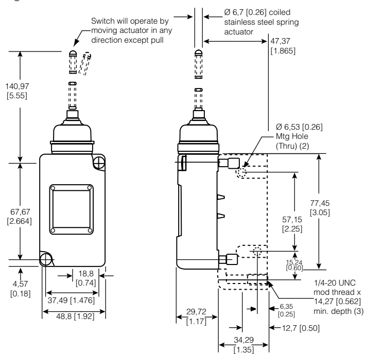
Figure 23. 208LS152 Dimensions
