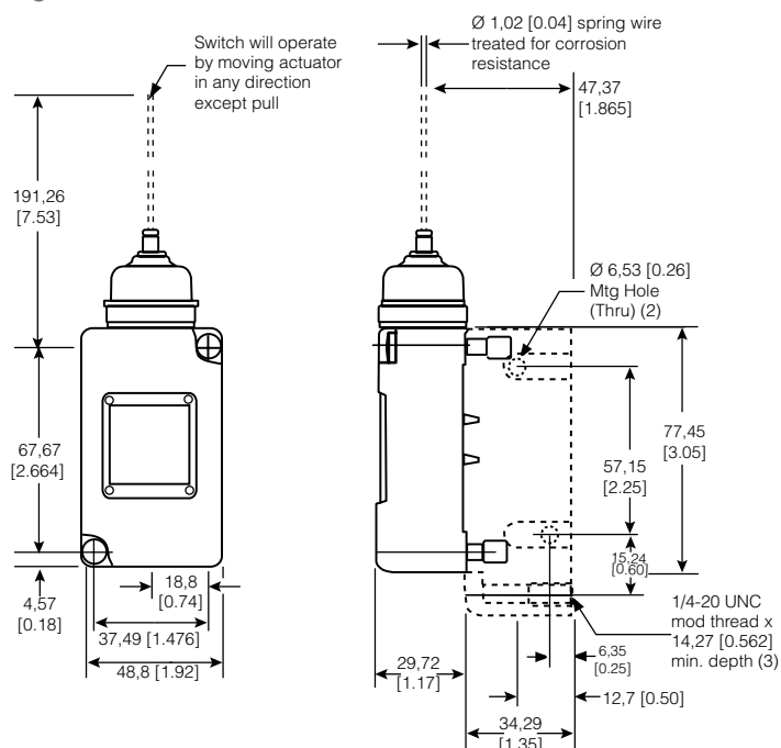
Figure 22. 208LS125 Dimensions
