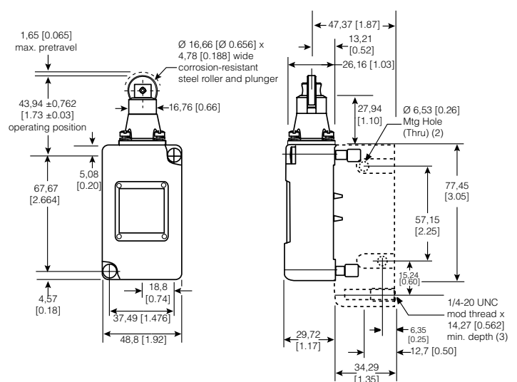
Figure 19. 206LS1 Dimensions
