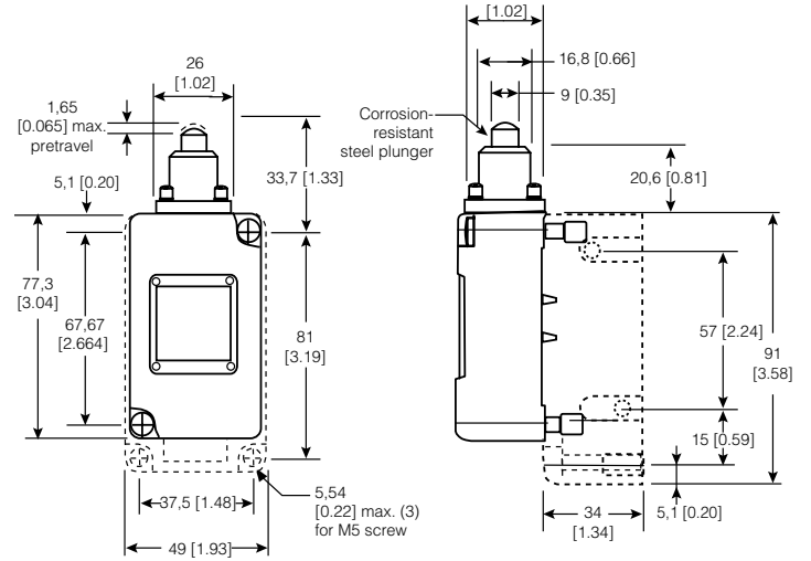
Figure 39. 208LS1-4 Dimensions
