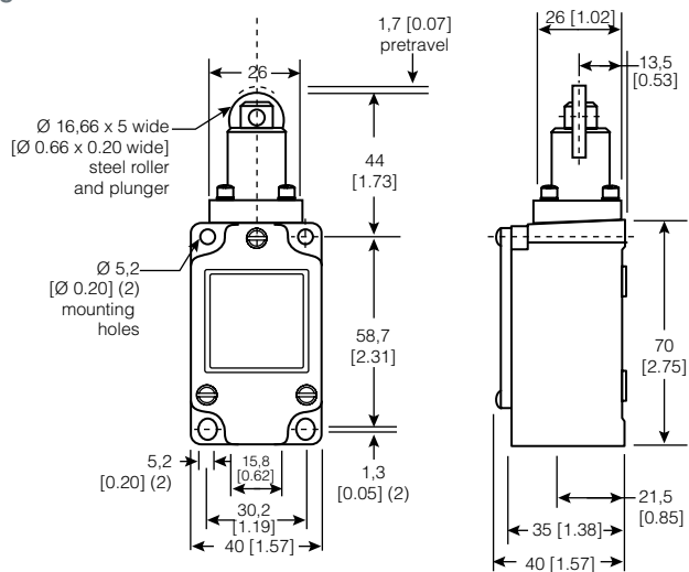
Figure 30. 6LS1-4 Dimensions
