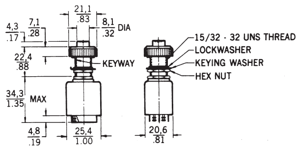
Watertight Switch
