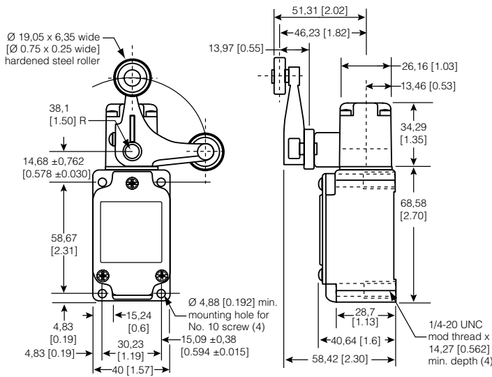
Figure 6. 6LS1 Dimensions
