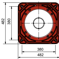
BURNER FLANGE
