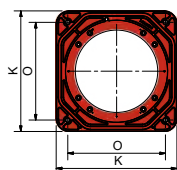
BURNER FLANGE
