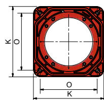
BURNER FLANGE
