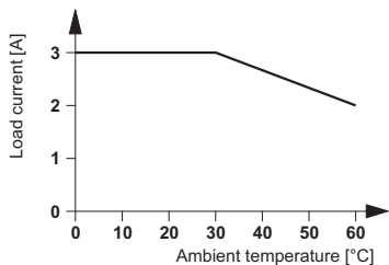
Derating curve for SIM-EI-OV-24 DC/24 DC/3
