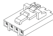
Mating Connector for 841408xxx and 841409xxx Molex # 50-57-9404 without pins Crimp Pins Molex # 16-02-0103
