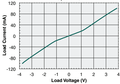
Load Current vs. Load Voltage ( I_F=0mA )
