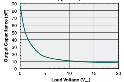
Output Capacitance vs. Load Voltage ( I_F=2mA )
