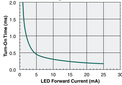
Turn-On Time vs. LED Forward Current ( I_L=80mA )
