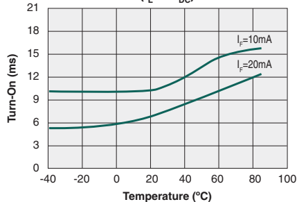
Typical Turn-On vs. Temperature ( I_L=1\text{A}_{DC} )
