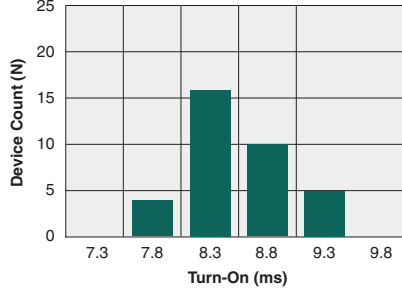
Typical Turn-On Time (N=35, I_F=20\text{mA} , I_L=1\text{A}_{DC} , T_A=25^\circ\text{C} )
