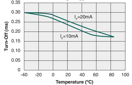
Typical Turn-Off vs. Temperature ( I_L=1\text{A}_{DC} )
