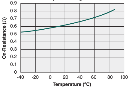
Typical On-Resistance vs. Temperature ( I_F=20\text{mA} , I_L=1\text{A} )
