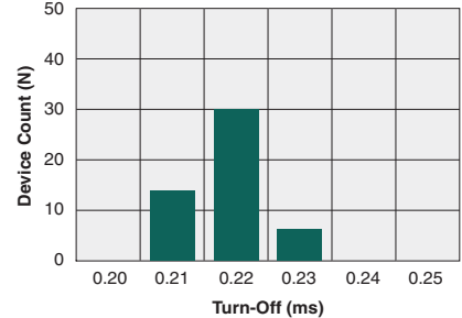
Typical Turn-Off Time (N=50, I_F=20\text{mA} , I_L=1\text{A}_{DC} , T_A=25^\circ\text{C} )
