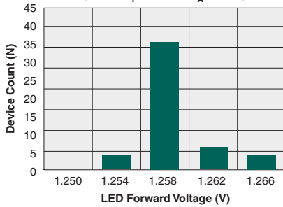
Typical LED Forward Voltage Drop ( N=50, I_F=10mA, T_A=25^\circ C )
