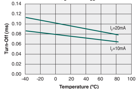
Typical Turn-Off vs. Temperature ( I_L=100mA_{DC} )
