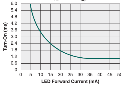
Typical Turn-On vs. LED Forward Current ( I_L=100mA_{DC} )
