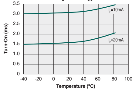
Typical Turn-On vs. Temperature ( I_L=100mA_{DC} )
