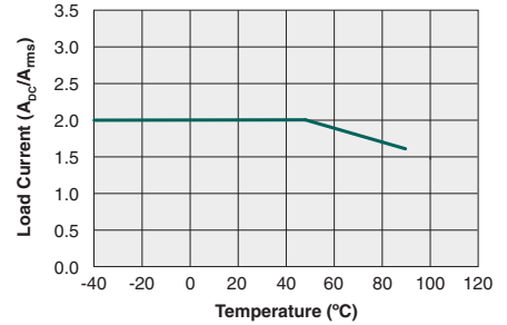
Maximum Load Current vs. Temperature ( I_F=10\text{mA} )
