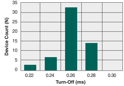
Typical Turn-Off Time (N=50, I_F=2mA , I_L=90mA_{DC} , T_A=25^\circ C )
