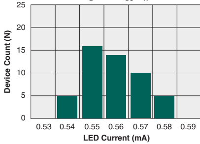
Typical I_F for Switch Operation (N=50, I_L=90mA_{DC} , T_A=25^\circ C )
