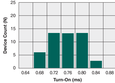
Typical Turn-On Time (N=50, I_F=2mA , I_L=90mA_{DC} , T_A=25^\circ C )
