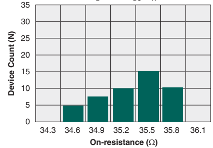
Typical On-Resistance Distribution (N=50, I_L=90mA_{DC} , T_A=25^\circ C )
