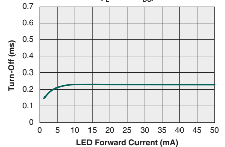
Typical Turn-Off vs. LED Forward Current ( I_L=90mA_{DC} )
