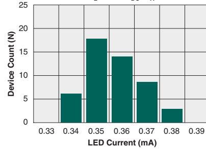
Typical I_F for Switch Dropout (N=50, I_L=90mA_{DC} , T_A=25^\circ C )
