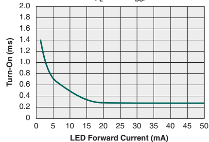
Typical Turn-On vs. LED Forward Current ( I_L=90mA_{DC} )
