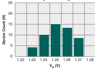
Typical V_{IN} for Switch Operation (N=50, I_L=100mA , T_A=25^\circ C )
