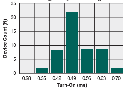
Typical Turn-On Time (N=50, V_{IN}=5V , I_L=100mA , T_A=25^\circ C )
