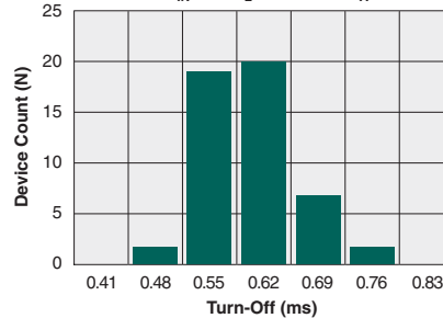
Typical Turn-Off Time (N=50, V_{IN}=5V , I_L=100mA , T_A=25^\circ C )
