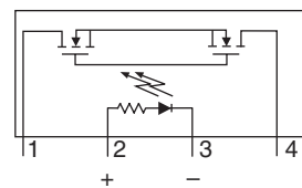
CPC1217 Pinout
