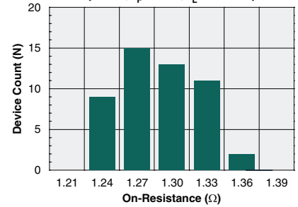
Typical On-Resistance Distribution (N=50, I_F=0\text{mA} , I_L=400\text{mA} )
