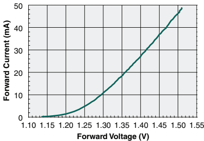
LED Forward Voltage vs. LED Forward Current
