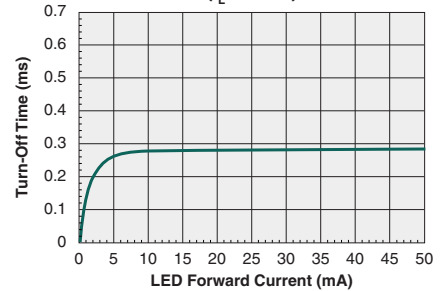
Typical Turn-Off Time vs. LED Forward Current (I L =80mA)
