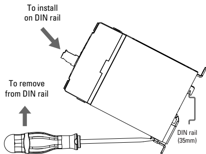
fig. 1 SSR mounted on DIN rail
