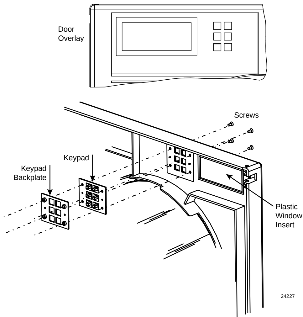
Figure 1 – Component Location
