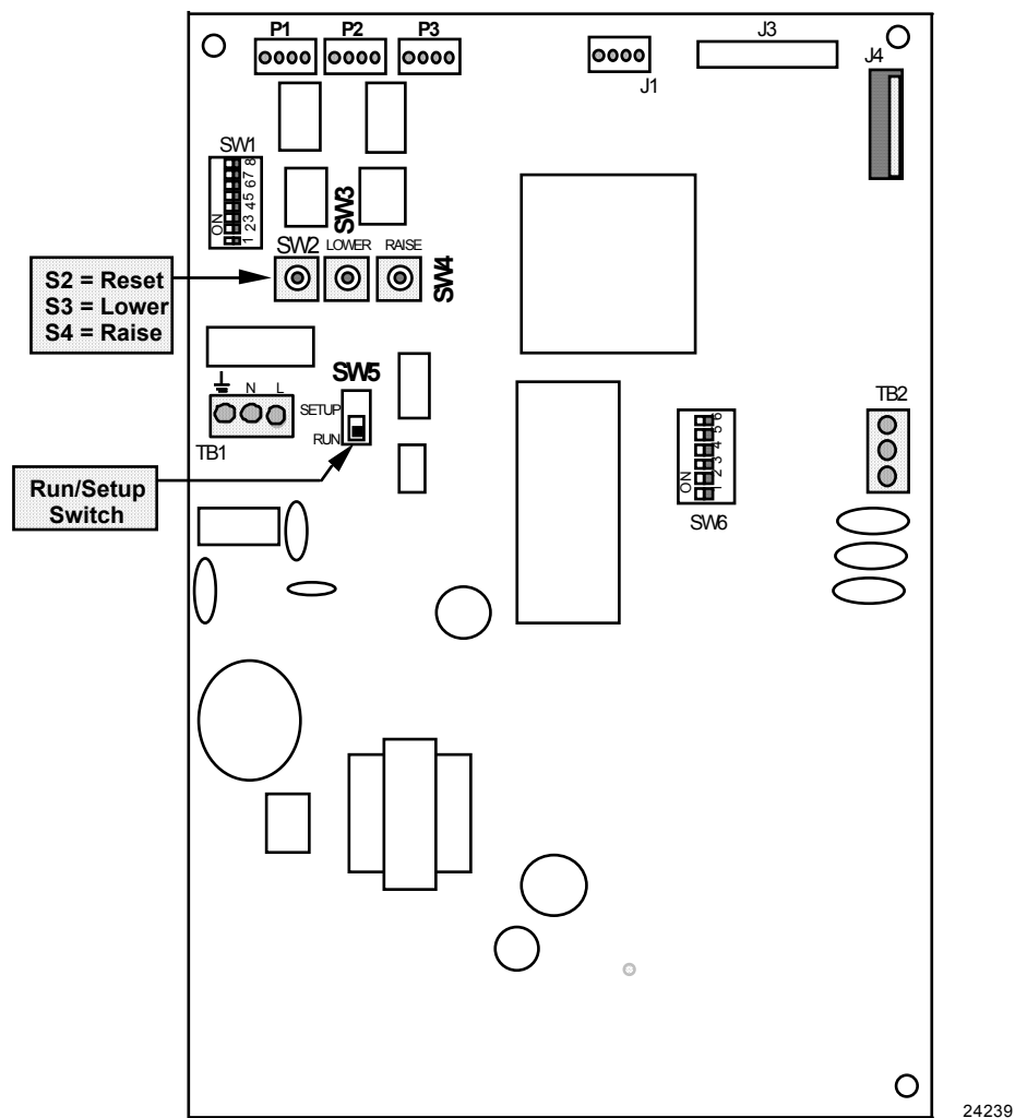
Figure 2 – Location of Switches
