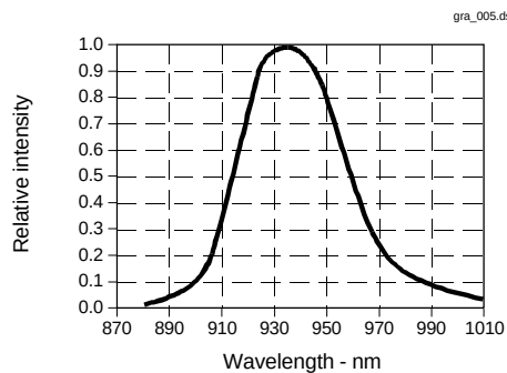
Fig. 5 Spectral Bandwidth
