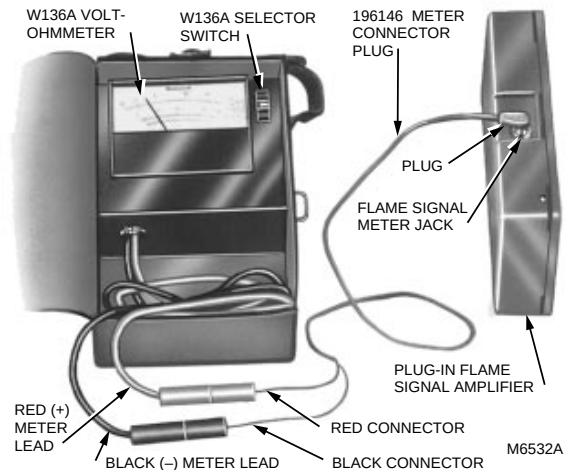
Fig. 17. Measuring microamp flame signal.
