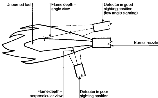
Fig. 5. Sighting angle
