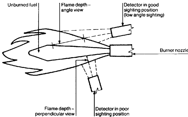
Fig. 5. Sighting angle
