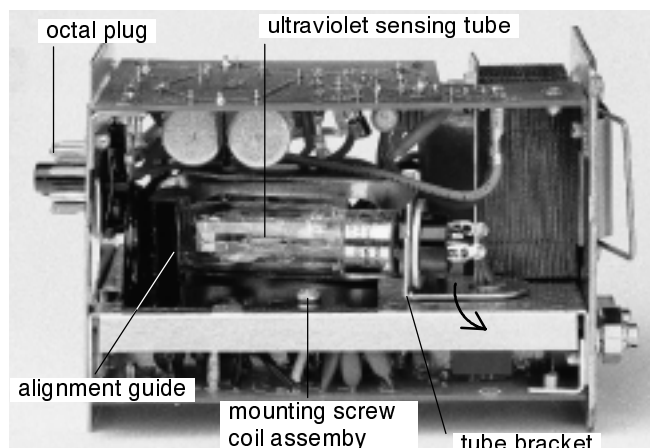
Fig. 19. Top view plug-in electronic chassis
