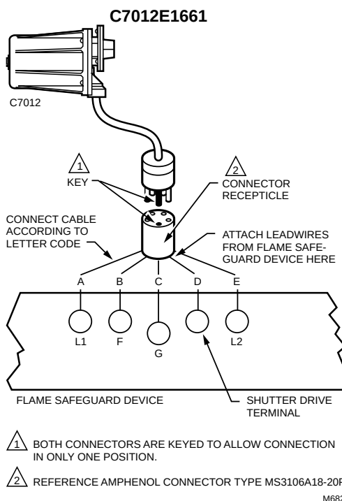
Fig. 16. Wiring connection for C7012E1161 or C7012E1278.
