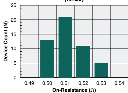
Typical On-Resistance Distribution (N=50)
