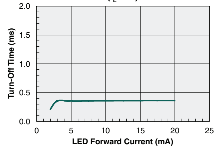
Typical Turn-Off Time vs. LED Forward Current ( I_L=1\text{A} )
