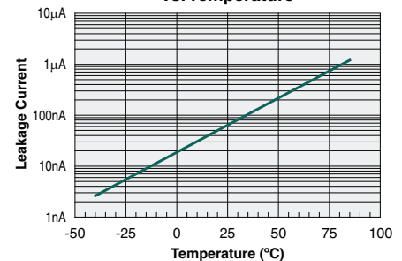
Typical Leakage Current vs. Temperature
