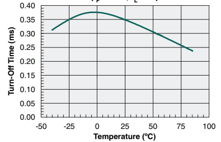
Typical Turn-Off Time vs. Temperature ( I_F=5\text{mA} , I_L=1\text{A} )
