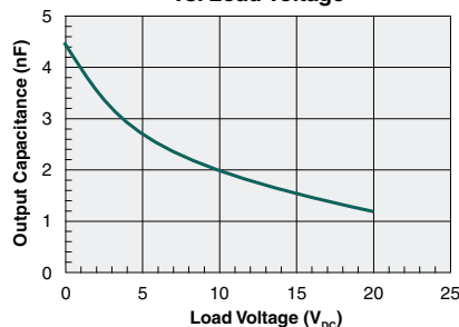
Typical Output Capacitance vs. Load Voltage
