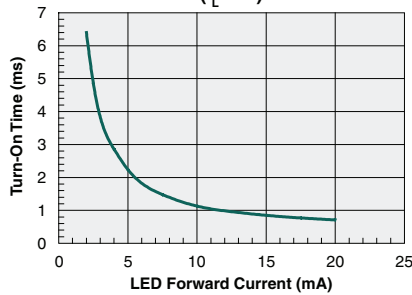
Typical Turn-On Time vs. LED Forward Current ( I_L=1\text{A} )
