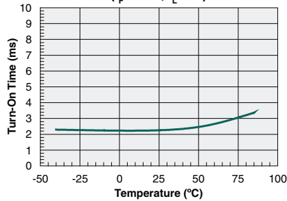
Typical Turn-On Time vs. Temperature ( I_F=5\text{mA} , I_L=1\text{A} )
