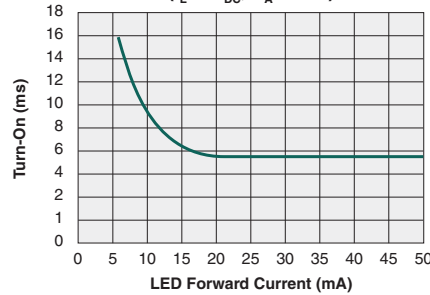
Typical Turn-On vs. LED Forward Current ( I_L=1\text{A}_{DC} , T_A=25^\circ\text{C} )
