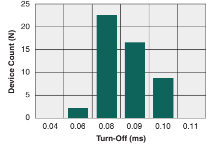
Typical Turn-Off Time (N=50, I_F=10\text{mA} , I_L=1\text{A}_{DC} , T_A=25^\circ\text{C} )
