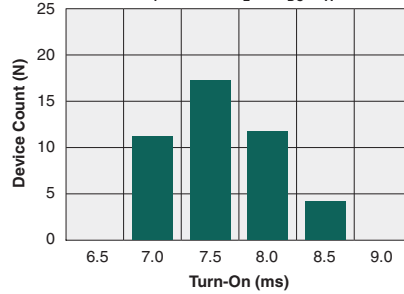
Typical Turn-On Time (N=50, I_F=10\text{mA} , I_L=1\text{A}_{DC} , T_A=25^\circ\text{C} )
