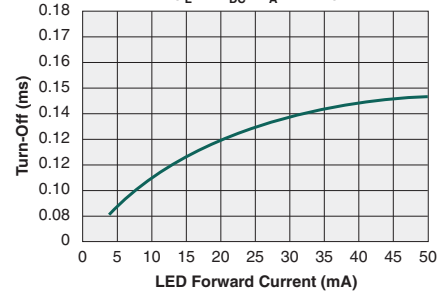
Typical Turn-Off vs. LED Forward Current ( I_L=1\text{A}_{DC} , T_A=25^\circ\text{C} )
