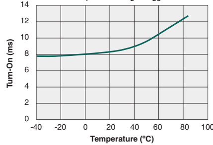
Typical Turn-On vs. Temperature ( I_F=10\text{mA} , I_L=1\text{A}_{DC} )
