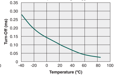
Typical Turn-Off vs. Temperature ( I_F=10\text{mA} , I_L=1\text{A}_{DC} )
