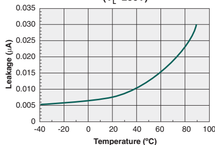
Typical Leakage vs. Temperature
