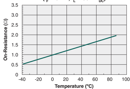
Typical On-Resistance vs. Temperature
