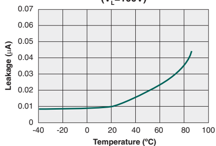
Typical Leakage vs. Temperature at Measured across Pins 3 & 4 ( V_L=100V )
