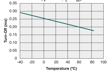
Typical Turn-Off vs. Temperature ( I_F=10\text{mA} , I_L=1A_{DC} )
