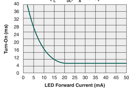
Typical Turn-On vs. LED Forward Current ( I_L=1A_{DC} , T_A=25^\circ\text{C} )
