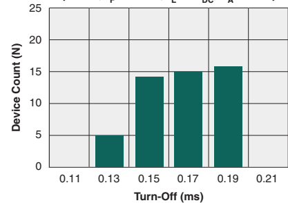
Typical Turn-Off Time ( N=50 , I_F=10\text{mA} , I_L=1A_{DC} , T_A=25^\circ\text{C} )
