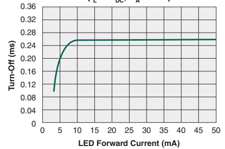
Typical Turn-Off vs. LED Forward Current ( I_L=1A_{DC} , T_A=25^\circ\text{C} )
