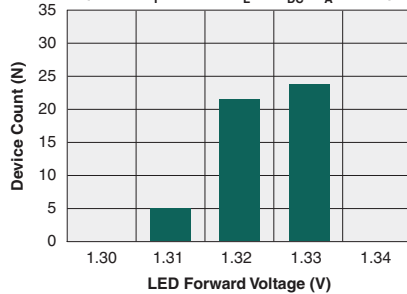
Typical LED Forward Voltage Drop ( N=50 , I_F=10\text{mA} , I_L=1A_{DC} , T_A=25^\circ\text{C} )
