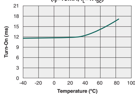
Typical Turn-On vs. Temperature ( I_F=10\text{mA} , I_L=1A_{DC} )
