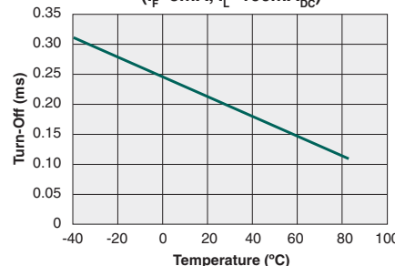
Typical Turn-Off vs. Temperature ( I_F=5\text{mA} , I_L=100\text{mA}_{DC} )
