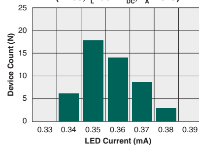
Typical I_F for Switch Dropout (N=50, I_L=90\text{mA}_{DC} , T_A=25^\circ\text{C} )
