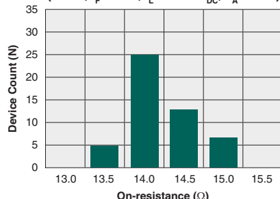
Typical On-Resistance Distribution (N=50, I_F=2\text{mA} , I_L=140\text{mA}_{DC} , T_A=25^\circ\text{C} )
