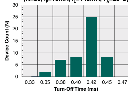
Typical Turn-Off Time (N=50, I_F=10\text{mA} , I_L=140\text{mA} , T_A=25^\circ\text{C} )
