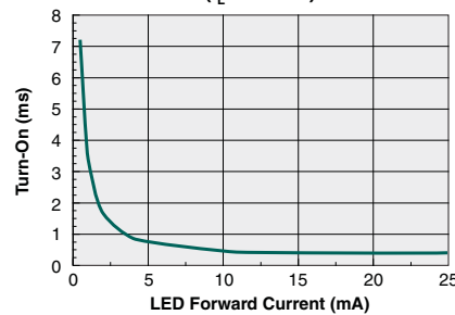
Typical Turn-On vs. LED Forward Current ( I_L=120\text{mA} )
