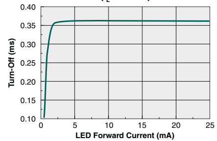
Typical Turn-Off vs. LED Forward Current ( I_L=120\text{mA} )
