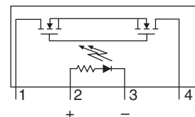
CPC1218 Pinout
