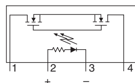
CPC1217 Pinout
