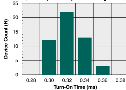
Typical Turn-On Time (N=50, I_F=2\text{mA} , I_L=100\text{mA} , T_A=25^\circ\text{C} )
