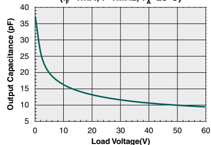
Output Capacitance vs. Load Voltage ( I_F=1\text{mA} , f=1\text{MHz} , T_A=25^{\circ}\text{C} )
